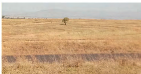
Figure 38: Abandoned lands around Assosa
