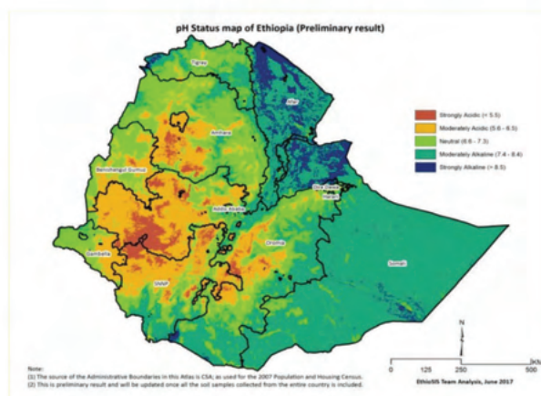
Figure 37: Geographical distribution of acid soil in Ethiopia (ATA, 2017)
